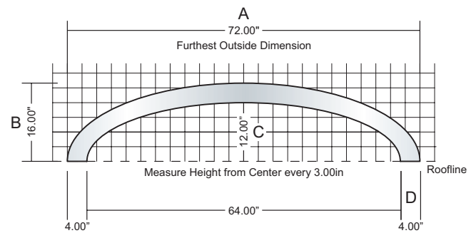
Frieze Board Type - Elliptical
