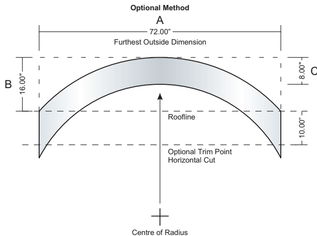
PVC Cladding Facade
