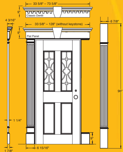
Pilaster Kit shown with 9" HEADERS
